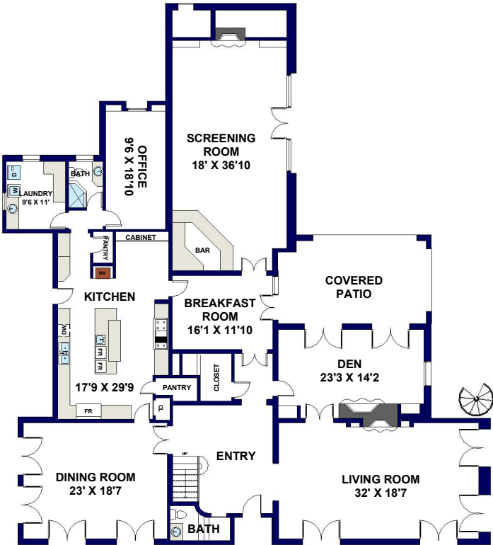
FIRST FLOOR
